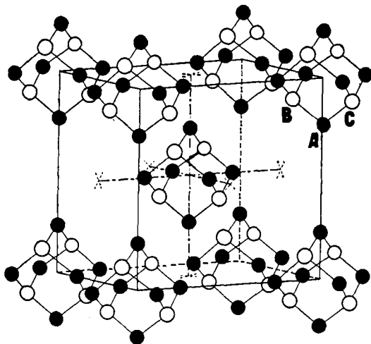
Fig. 3.—Arrangement of the carbon atoms (black circles) and nitrogen atoms (white circles) in C_6H_{12}N_4 crystals.
